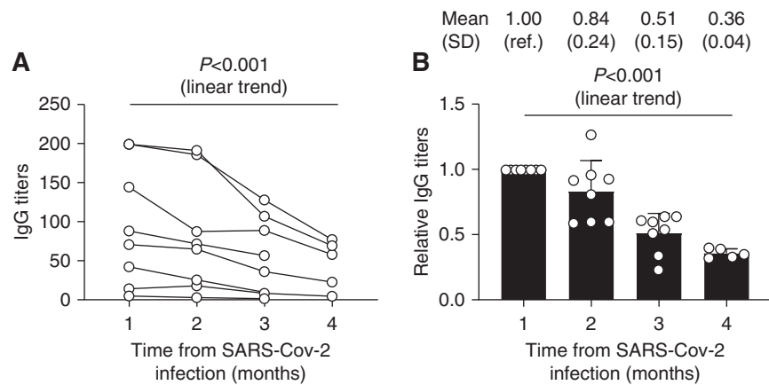
Figure 1. | Progressive decrease of anti-SARS-CoV-2 IgG levels over 3 months. Dynamic absolute (A) and relative (B) changes of antisevere acute respiratory syndrome coronavirus 2 (anti-SARS-CoV-2) IgG levels. IgG levels decreased significantly during follow-up. ref., reference.
