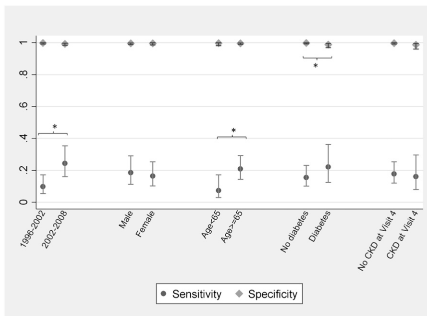
Figure 1. | The sensitivity and specificity of AKI billing codes vary according to patient characteristics and hospitalization year. Validated against chart review. Figure depicts point estimates and 95% confidence intervals. * P < 0.05 .
