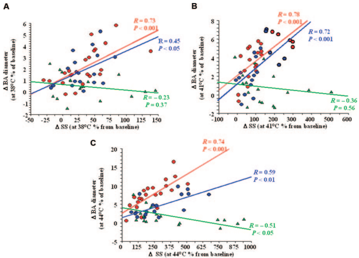
Figure 1. Relationships (adjusted for age and mean BP) between shear stress ( \Delta SS) and brachial artery ( \Delta BA) diameter changes at different hand-warming steps: (A) mild, (B) moderate, (C) high control subjects: red circles and regression lines; ESRD-CVD - patients: blue circles and regression lines; ESRD-CVD + patients: green triangles and regression lines.
