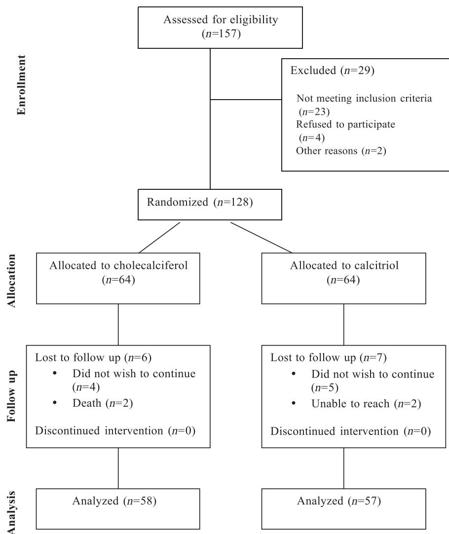
Figure 1. | Consort diagram.
